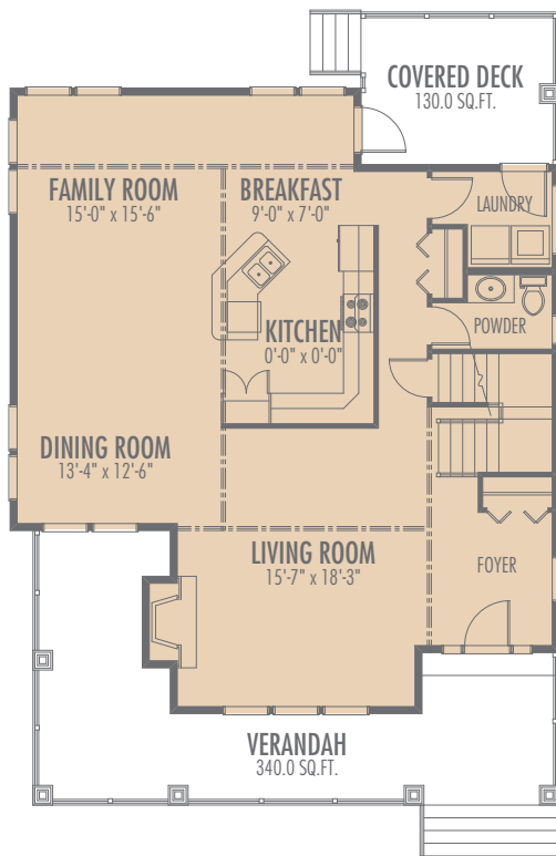
MAIN FLOOR
