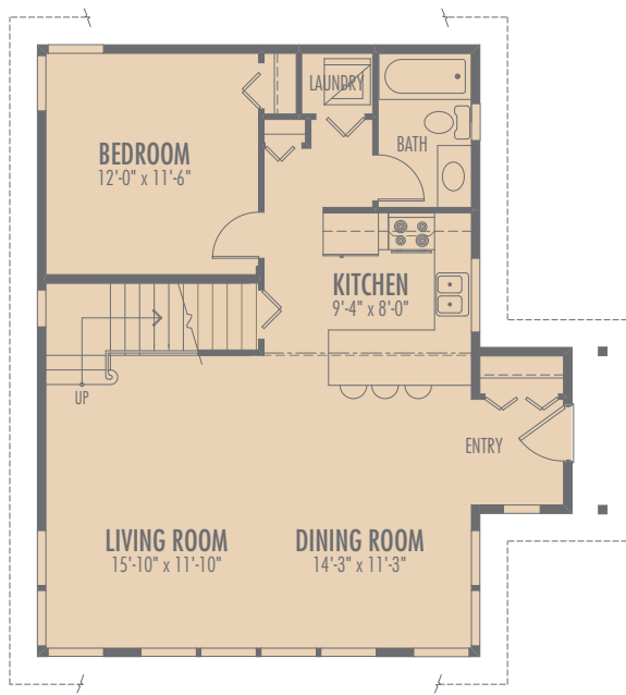
MAIN FLOOR
