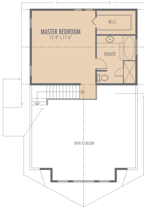
UPPER FLOOR
