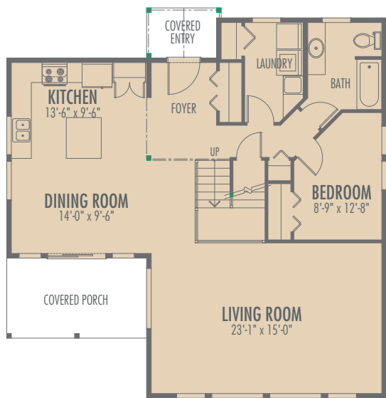
MAIN FLOOR
