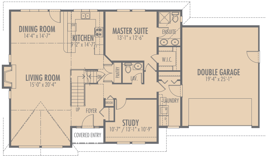
MAIN FLOOR
